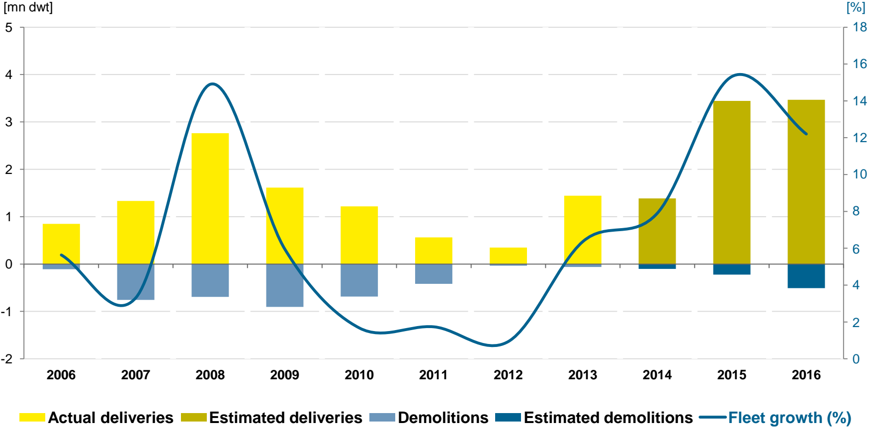
LPG tanker fleet development 2006-2016
